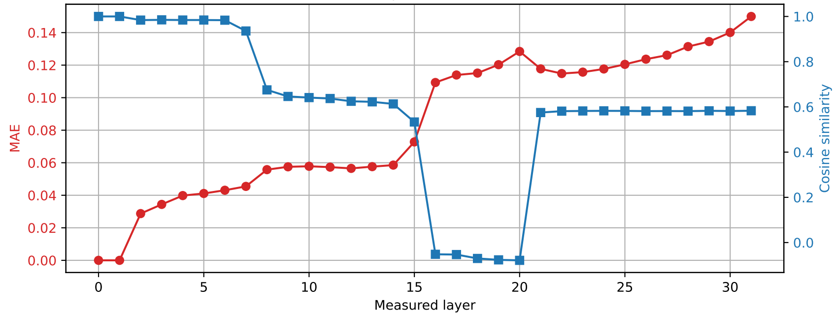
OLMo-7B-hf | Prompt 2 Spared layer 0 | Hybrid vs unquantized
