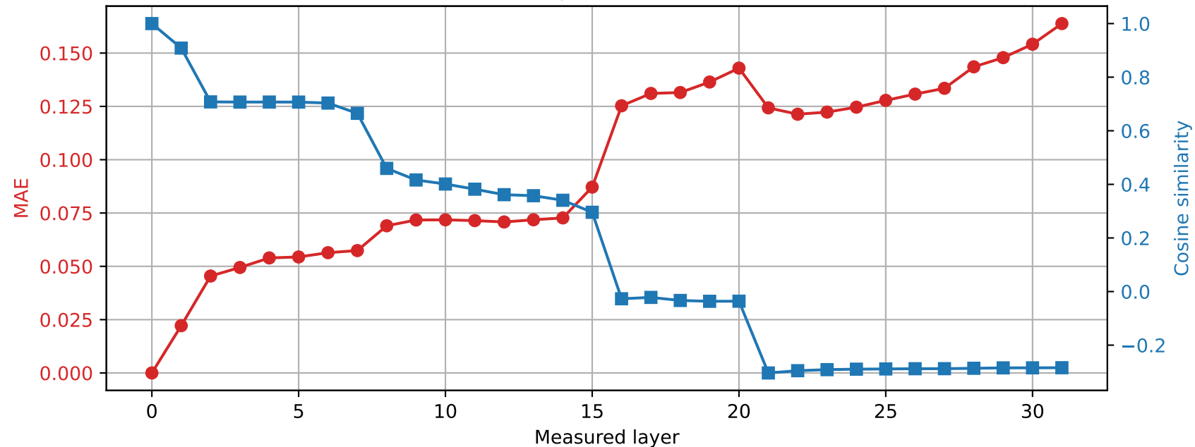
OLMo-7B-hf | Prompt 2 Spared layer 5 | Hybrid vs unquantized
