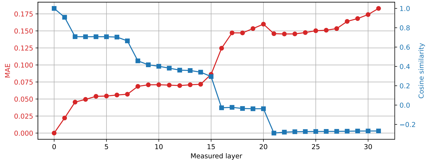
OLMo-7B-hf | Prompt 2 Spared layer 16 | Hybrid vs unquantized
