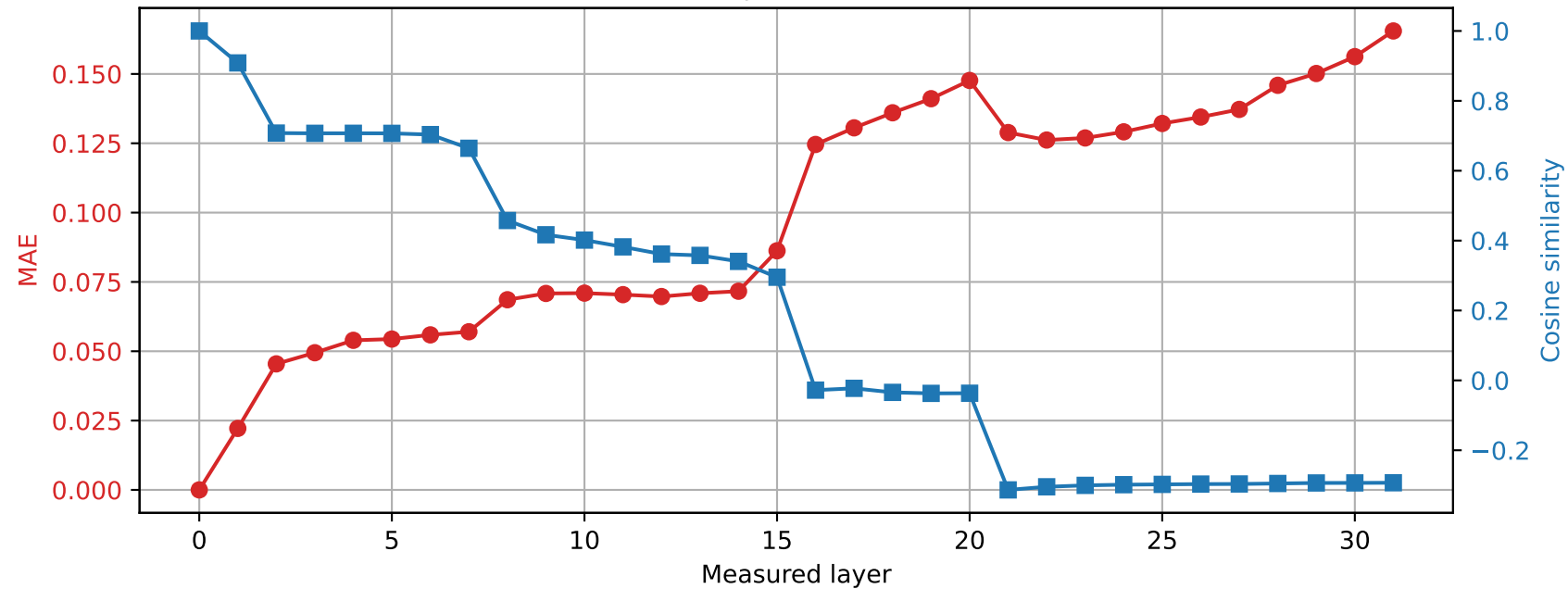
OLMo-7B-hf | Prompt 2 Spared layer 17 | Hybrid vs unquantized
