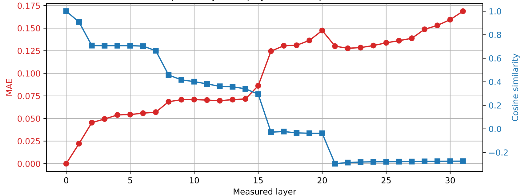
OLMo-7B-hf | Prompt 2 Spared layer 19 | Hybrid vs unquantized
