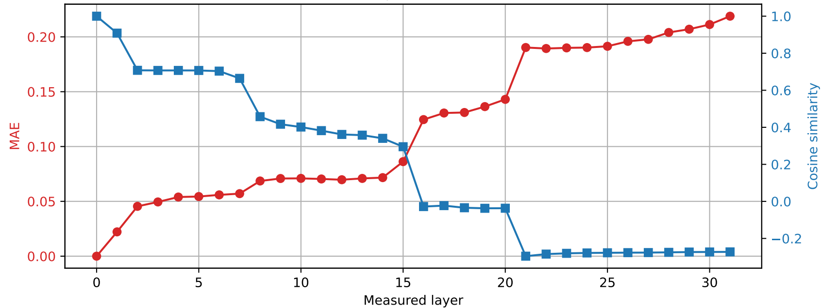
OLMo-7B-hf | Prompt 2 Spared layer 20 | Hybrid vs unquantized
