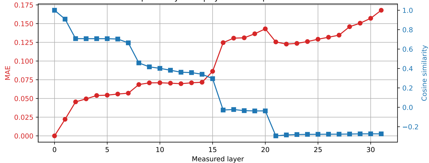
OLMo-7B-hf | Prompt 2 Spared layer 30 | Hybrid vs unquantized
