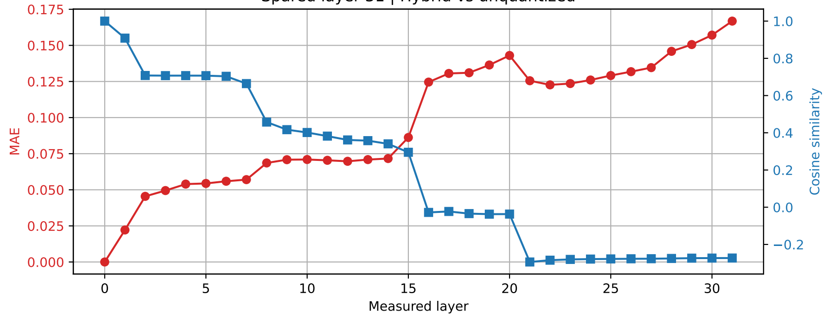
OLMo-7B-hf | Prompt 2 Spared layer 31 | Hybrid vs unquantized
