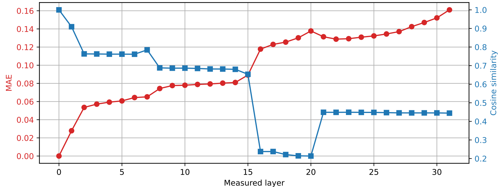
OLMo-7B-hf | Prompt 3 Spared layer 1 | Hybrid vs unquantized
