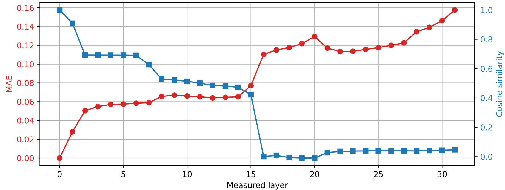
OLMo-7B-hf | Prompt 3 Spared layer 2 | Hybrid vs unquantized
