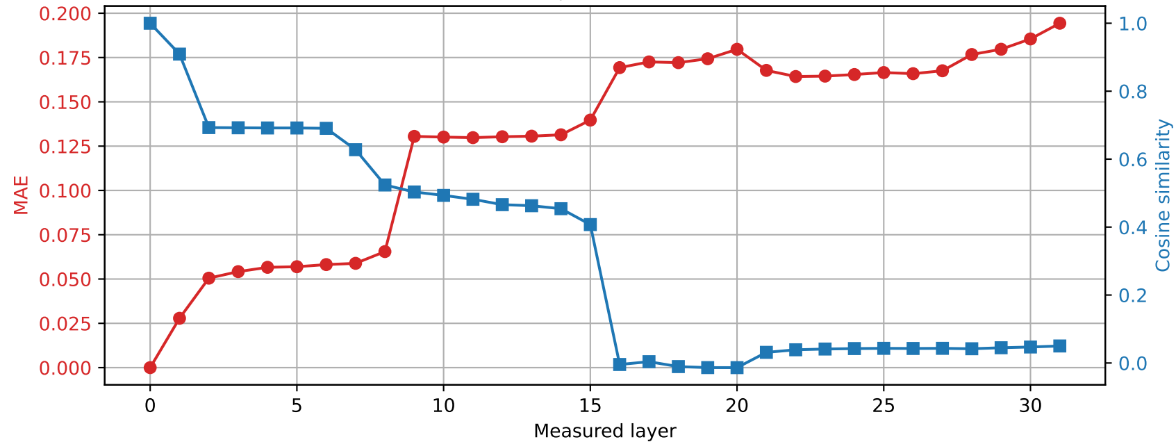
OLMo-7B-hf | Prompt 3 Spared layer 8 | Hybrid vs unquantized
