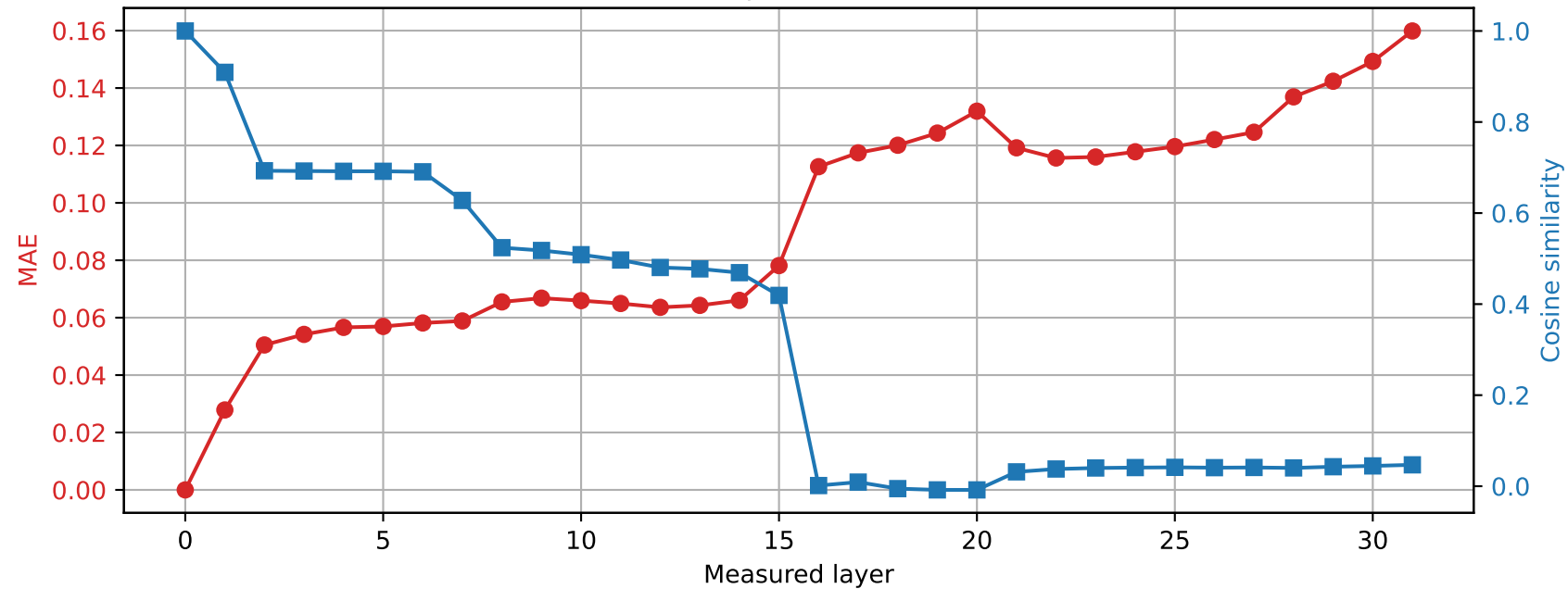
OLMo-7B-hf | Prompt 3 Spared layer 13 | Hybrid vs unquantized
