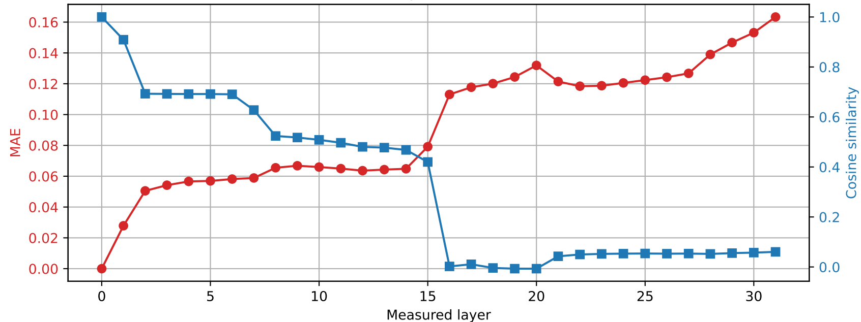
OLMo-7B-hf | Prompt 3 Spared layer 14 | Hybrid vs unquantized
