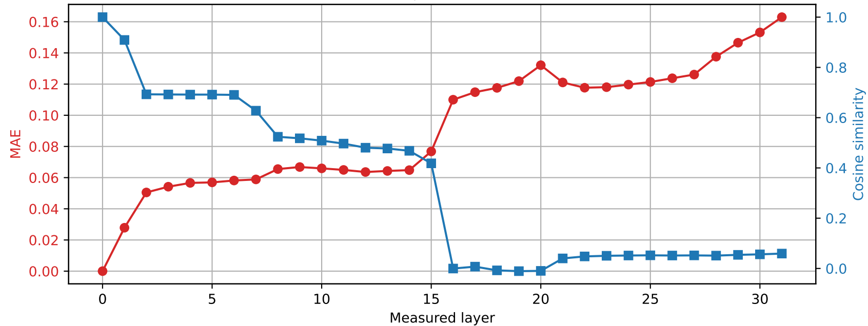
OLMo-7B-hf | Prompt 3 Spared layer 19 | Hybrid vs unquantized
