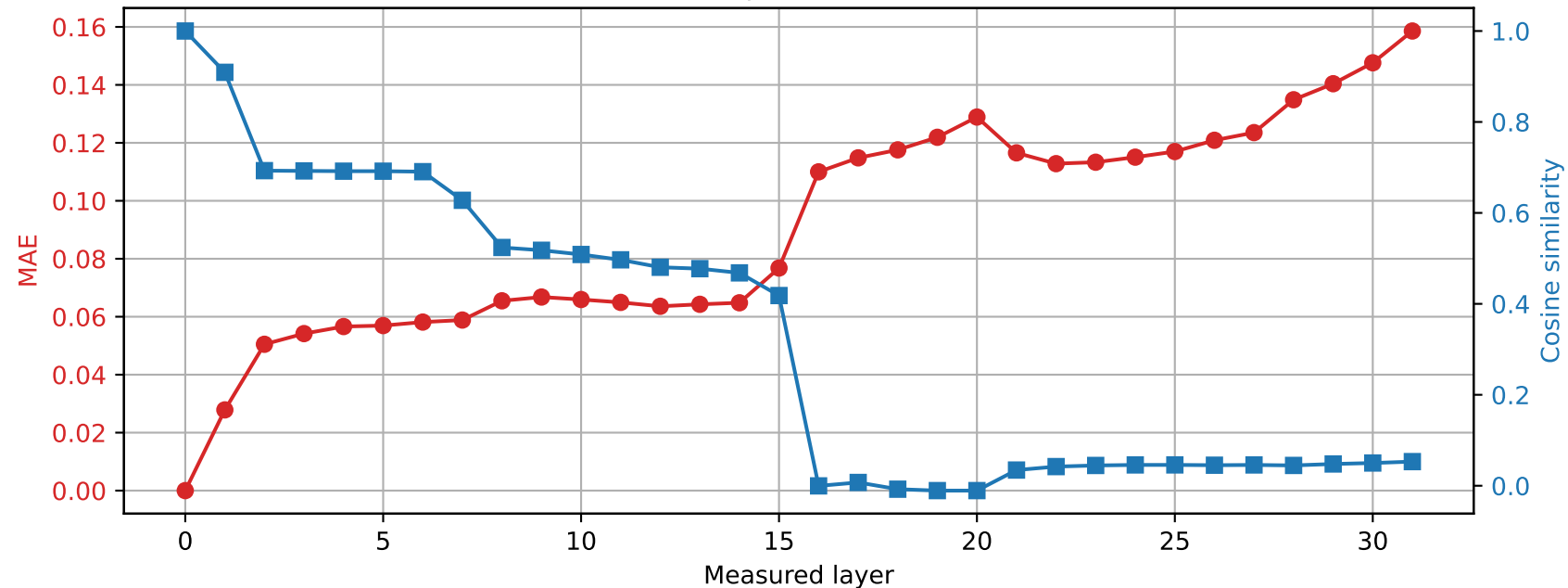
OLMo-7B-hf | Prompt 3 Spared layer 24 | Hybrid vs unquantized
