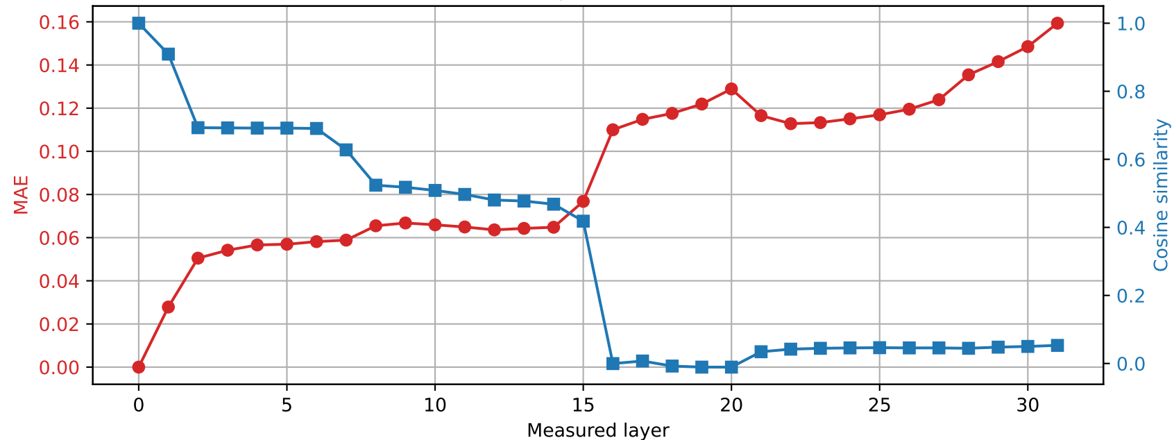
OLMo-7B-hf | Prompt 3 Spared layer 26 | Hybrid vs unquantized
