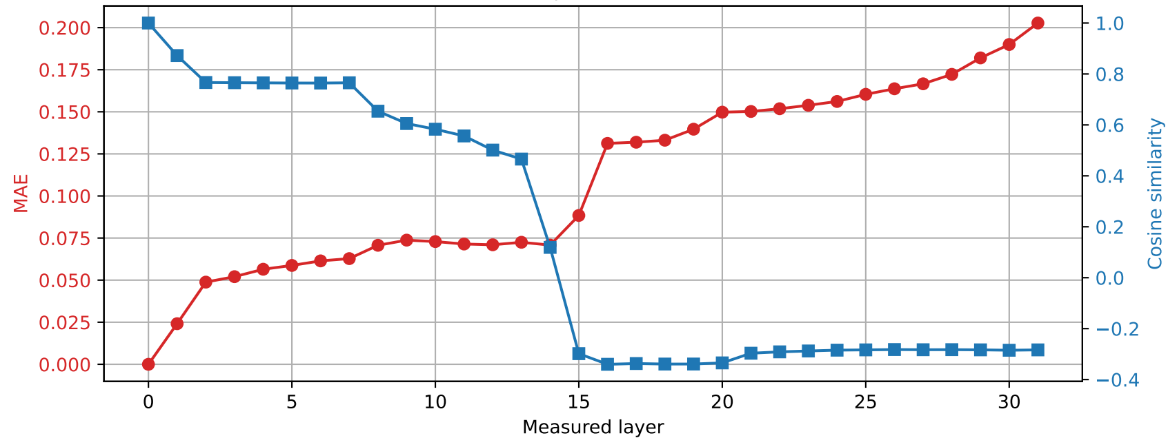
OLMo-7B-hf | Prompt 4 Spared layer 11 | Hybrid vs unquantized
