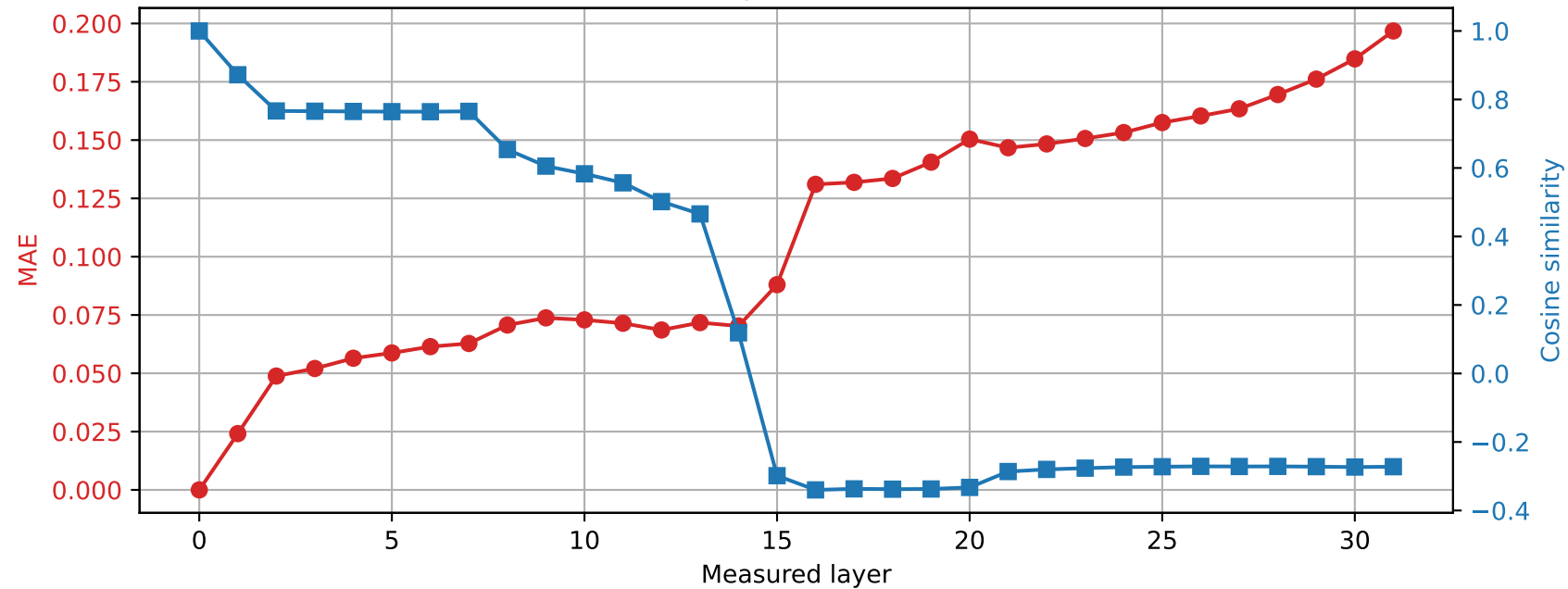
OLMo-7B-hf | Prompt 4 Spared layer 12 | Hybrid vs unquantized
