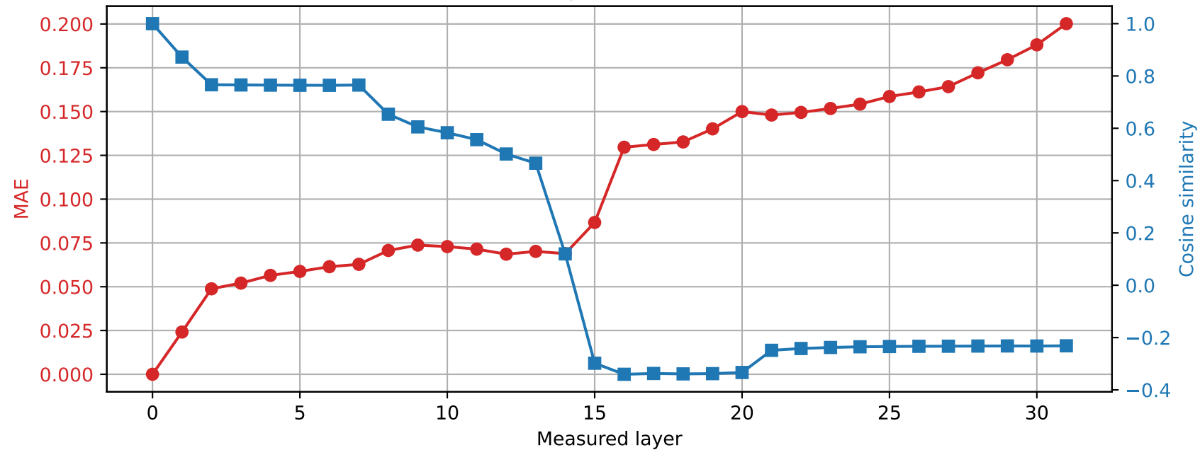
OLMo-7B-hf | Prompt 4 Spared layer 31 | Hybrid vs unquantized
