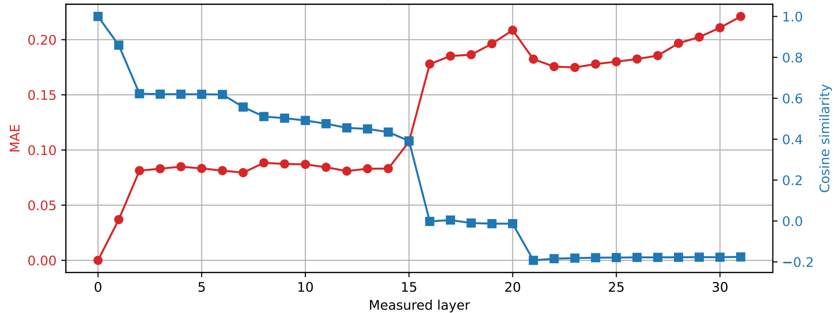
OLMo-7B-hf | Prompt 0 Spared layer 9 | Hybrid vs unquantized
