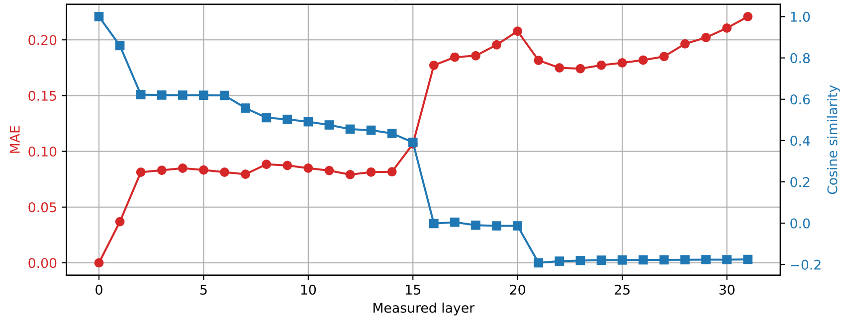
OLMo-7B-hf | Prompt 0 Spared layer 10 | Hybrid vs unquantized
