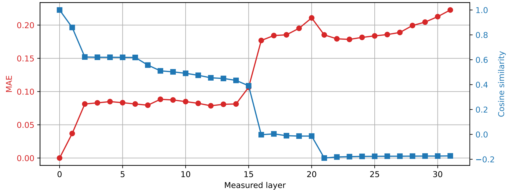
OLMo-7B-hf | Prompt 0 Spared layer 19 | Hybrid vs unquantized
