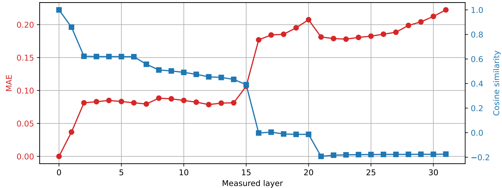
OLMo-7B-hf | Prompt 0 Spared layer 21 | Hybrid vs unquantized
