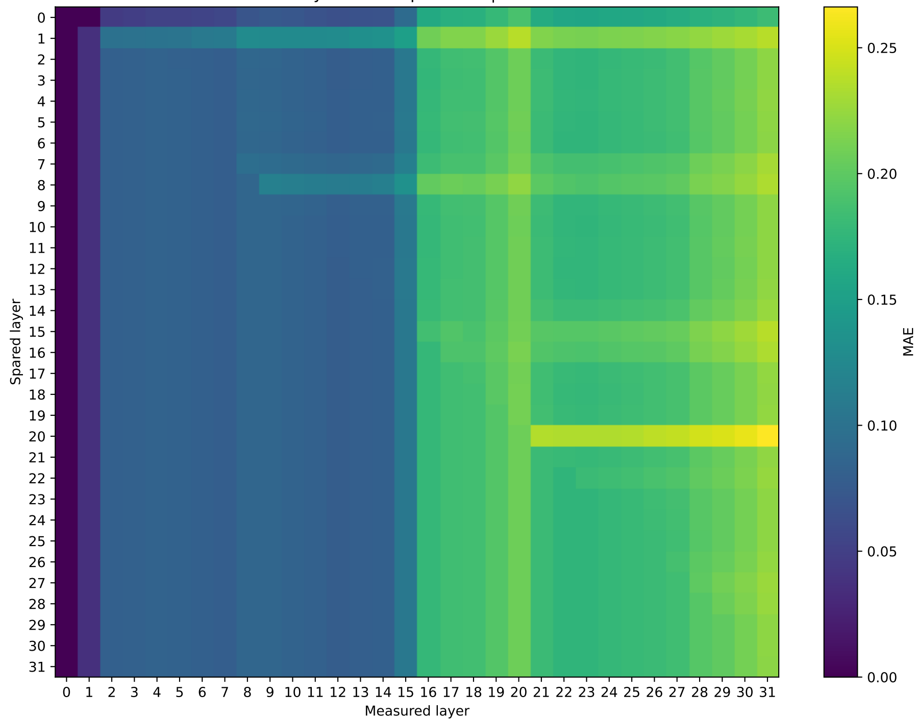
OLMo-7B-hf | Prompt 0 Hybrid vs unquantized | int4
