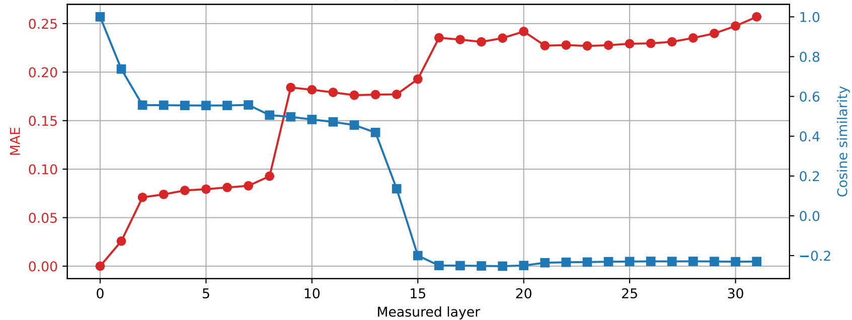
OLMo-7B-hf | Prompt 1 Spared layer 8 | Hybrid vs unquantized
