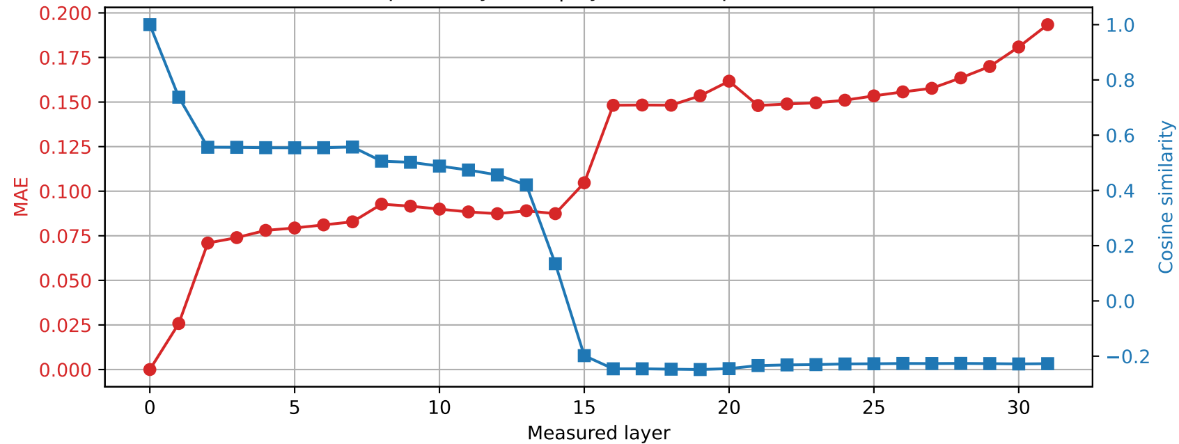
OLMo-7B-hf | Prompt 1 Spared layer 11 | Hybrid vs unquantized
