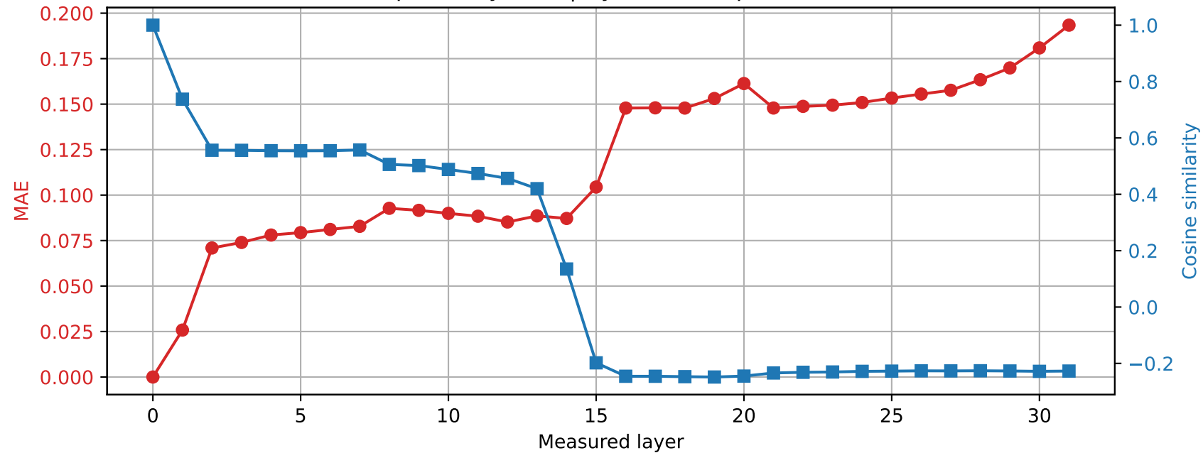
OLMo-7B-hf | Prompt 1 Spared layer 12 | Hybrid vs unquantized
