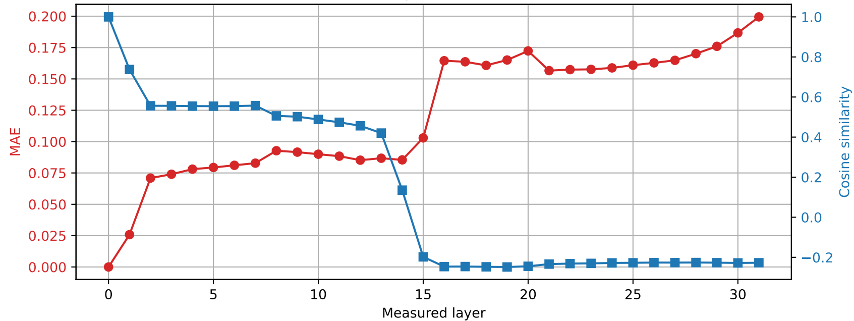
OLMo-7B-hf | Prompt 1 Spared layer 15 | Hybrid vs unquantized
