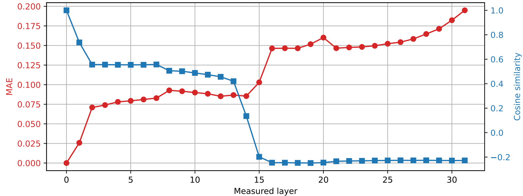
OLMo-7B-hf | Prompt 1 Spared layer 26 | Hybrid vs unquantized
