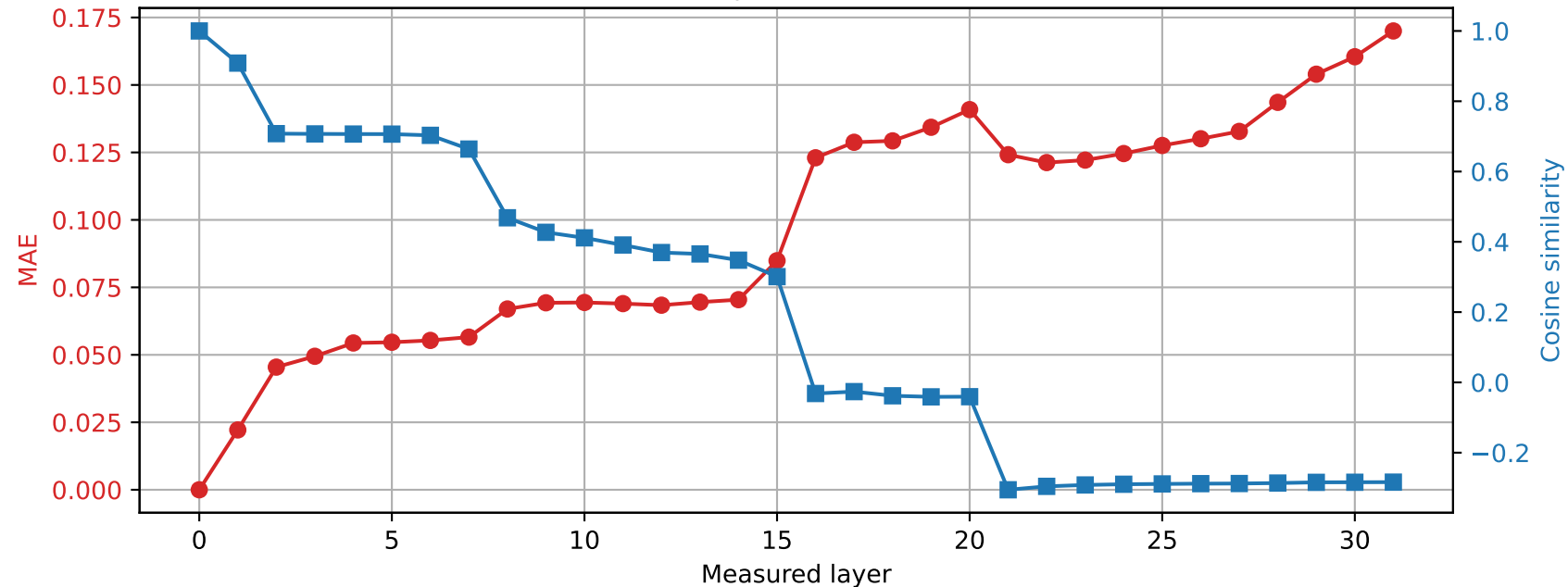
OLMo-7B-hf | Prompt 2 Spared layer 3 | Hybrid vs unquantized
