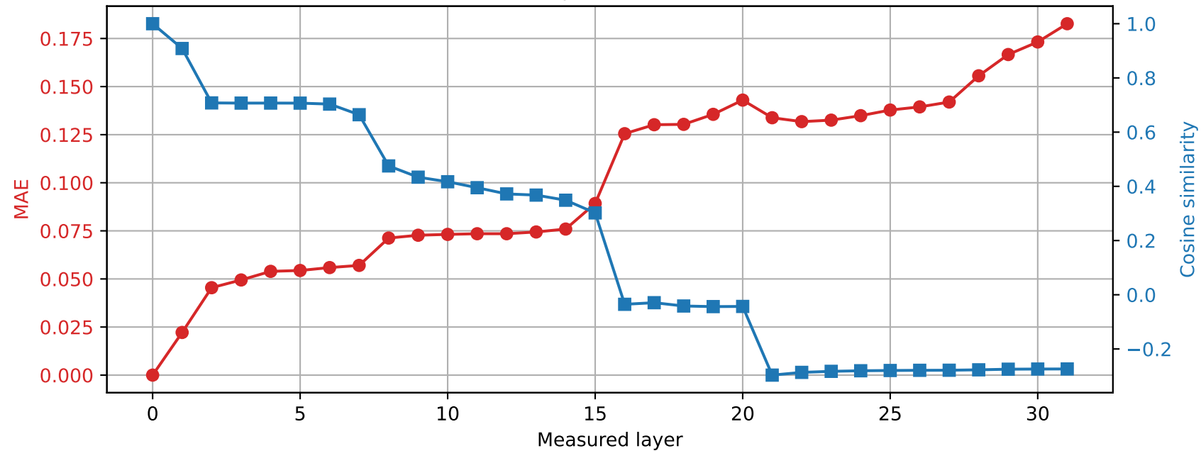
OLMo-7B-hf | Prompt 2 Spared layer 7 | Hybrid vs unquantized
