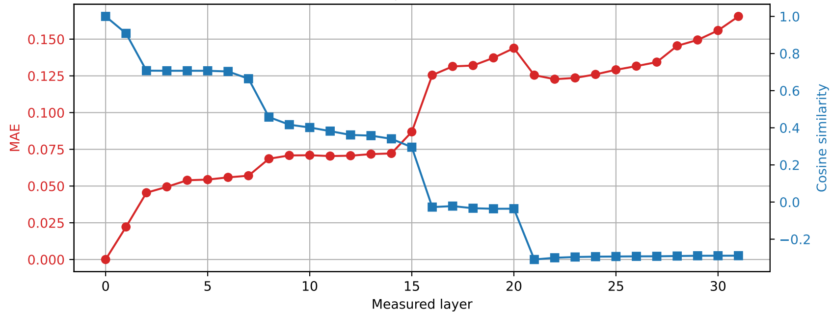
OLMo-7B-hf | Prompt 2 Spared layer 11 | Hybrid vs unquantized
