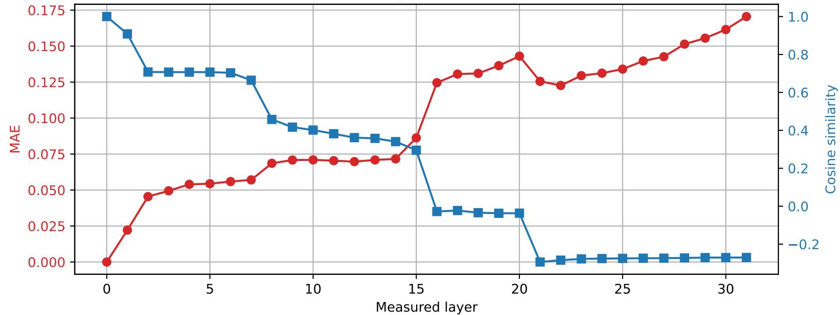
OLMo-7B-hf | Prompt 2 Spared layer 22 | Hybrid vs unquantized
