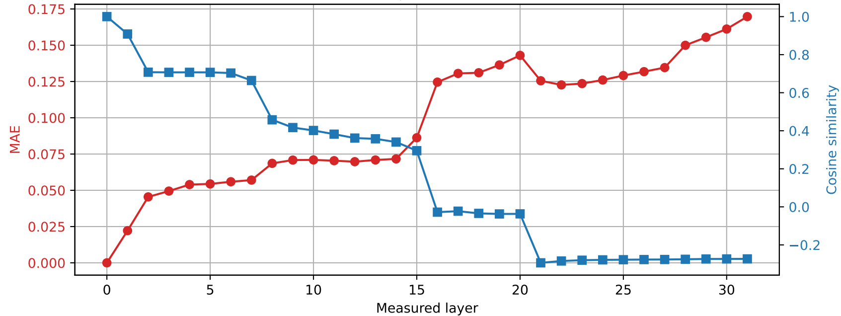
OLMo-7B-hf | Prompt 2 Spared layer 27 | Hybrid vs unquantized
