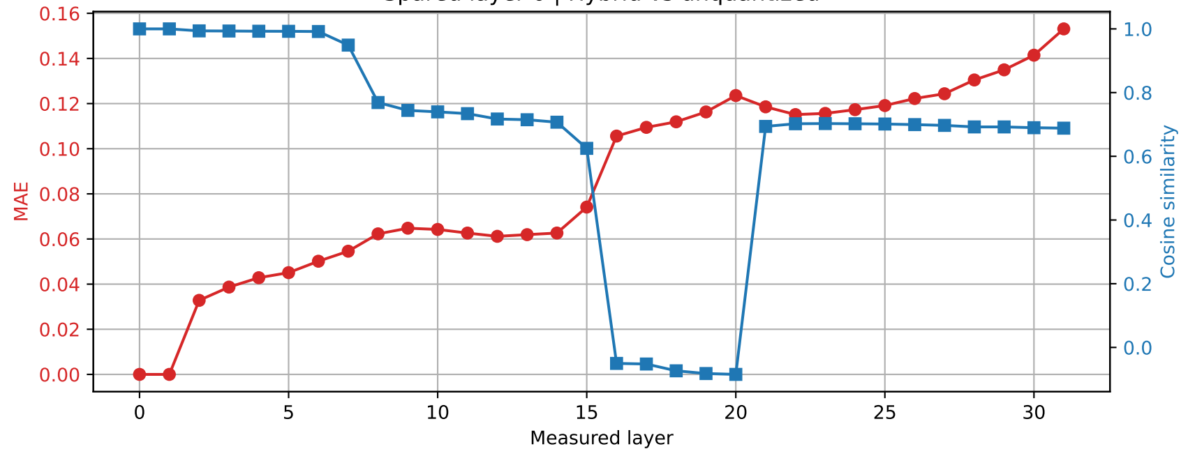
OLMo-7B-hf | Prompt 3 Spared layer 0 | Hybrid vs unquantized
