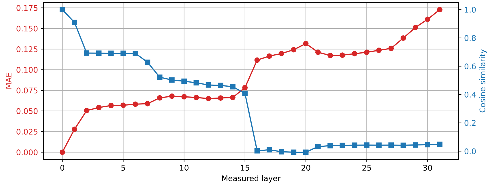
OLMo-7B-hf | Prompt 3 Spared layer 5 | Hybrid vs unquantized
