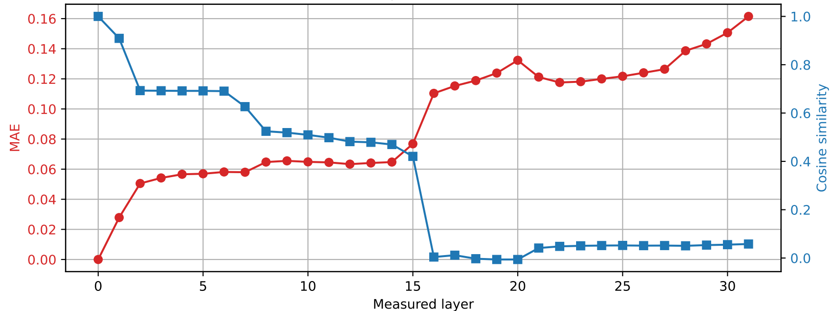
OLMo-7B-hf | Prompt 3 Spared layer 6 | Hybrid vs unquantized
