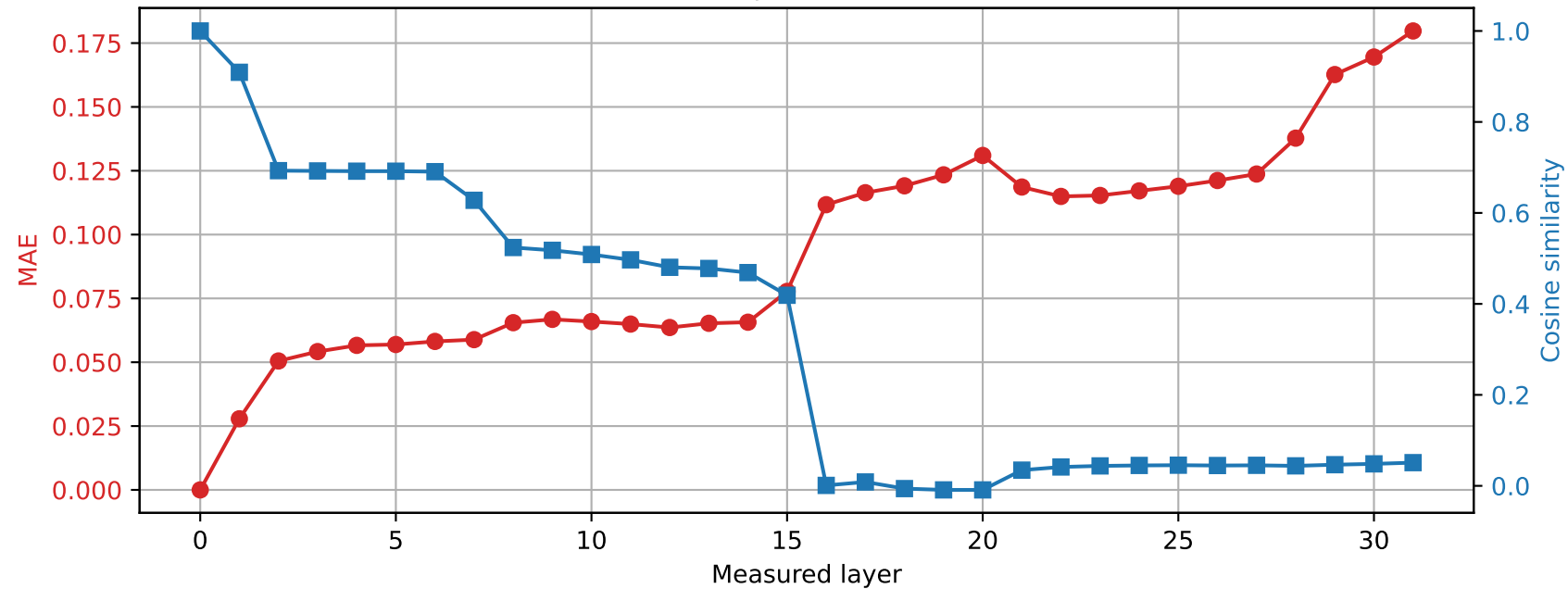
OLMo-7B-hf | Prompt 3 Spared layer 12 | Hybrid vs unquantized
