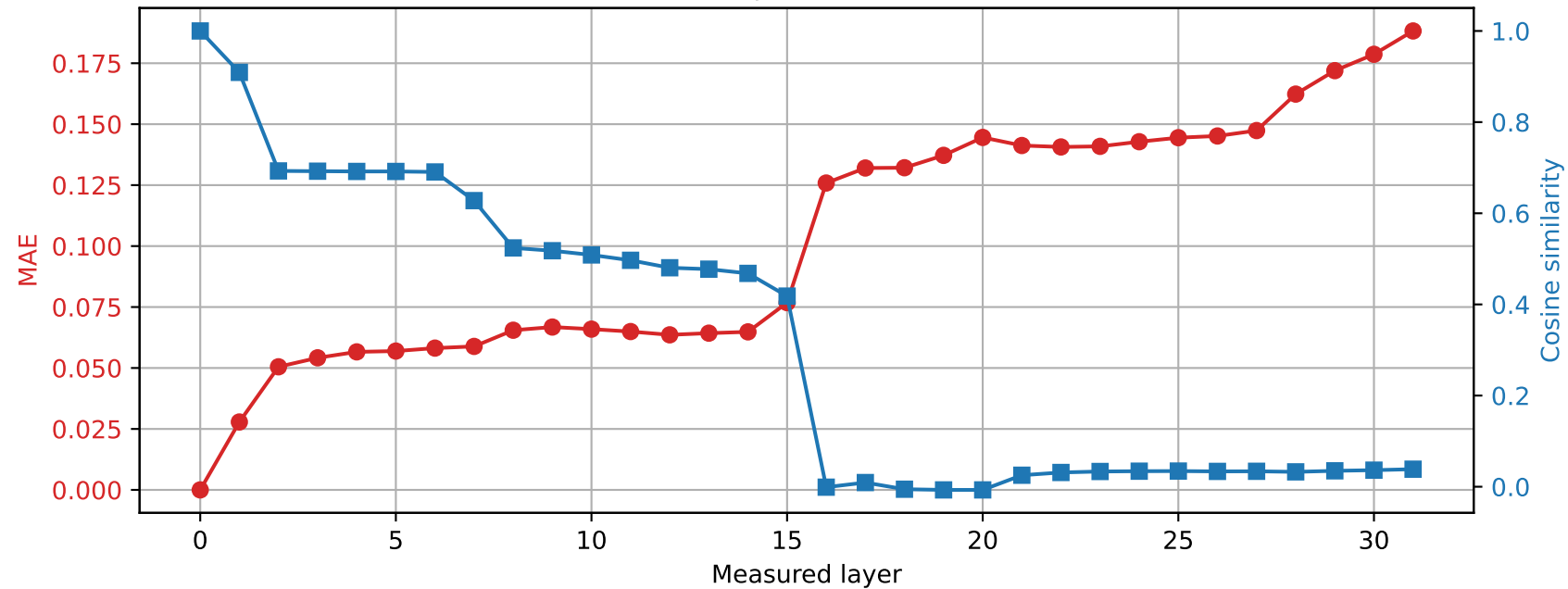
OLMo-7B-hf | Prompt 3 Spared layer 15 | Hybrid vs unquantized
