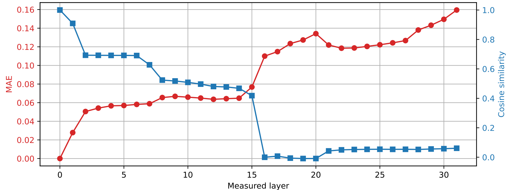
OLMo-7B-hf | Prompt 3 Spared layer 17 | Hybrid vs unquantized
