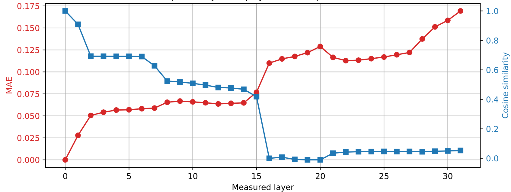
OLMo-7B-hf | Prompt 3 Spared layer 27 | Hybrid vs unquantized
