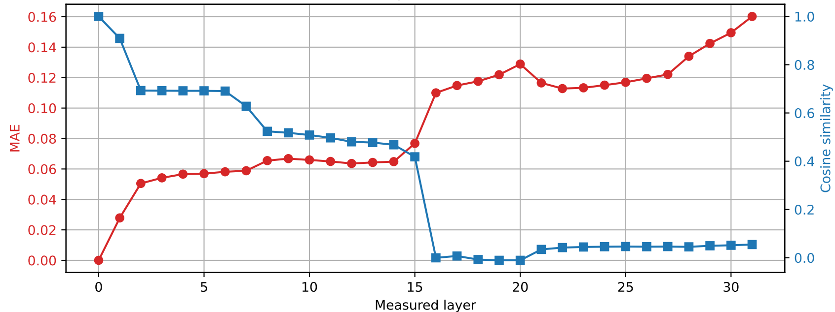
OLMo-7B-hf | Prompt 3 Spared layer 28 | Hybrid vs unquantized
