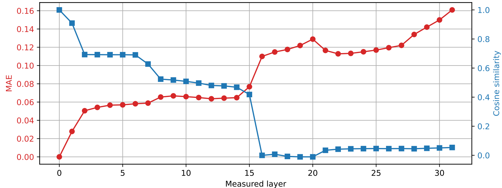
OLMo-7B-hf | Prompt 3 Spared layer 29 | Hybrid vs unquantized
