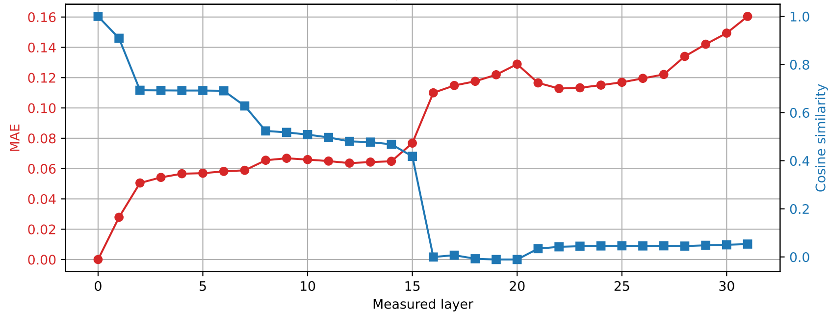
OLMo-7B-hf | Prompt 3 Spared layer 31 | Hybrid vs unquantized
