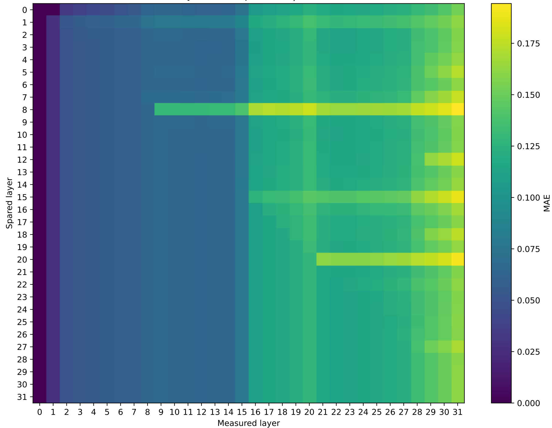
OLMo-7B-hf | Prompt 3 Hybrid vs unquantized | int4
