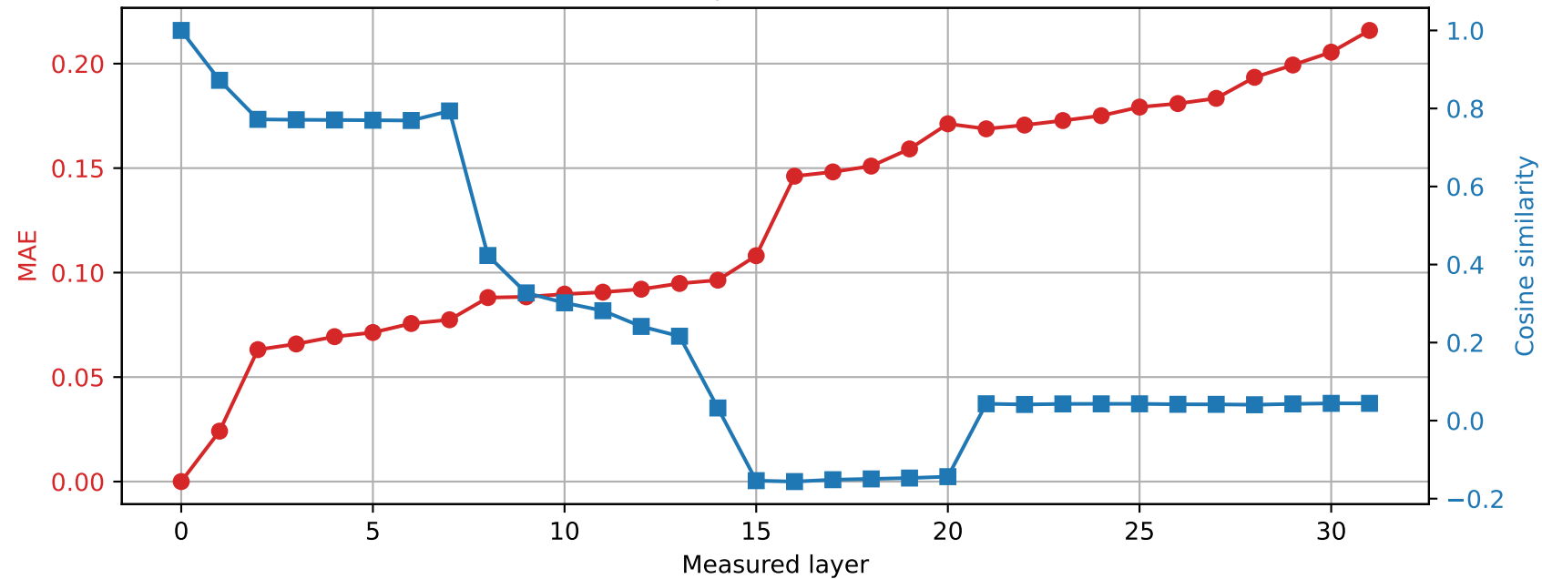
OLMo-7B-hf | Prompt 4 Spared layer 1 | Hybrid vs unquantized
