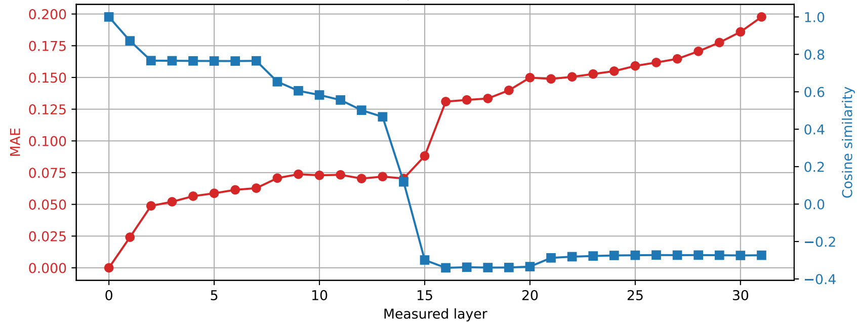
OLMo-7B-hf | Prompt 4 Spared layer 10 | Hybrid vs unquantized
