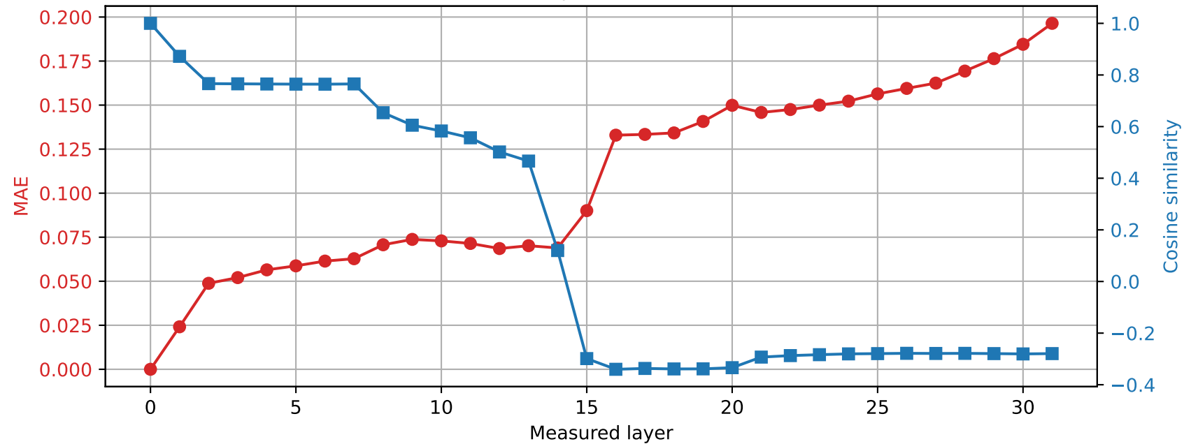
OLMo-7B-hf | Prompt 4 Spared layer 14 | Hybrid vs unquantized
