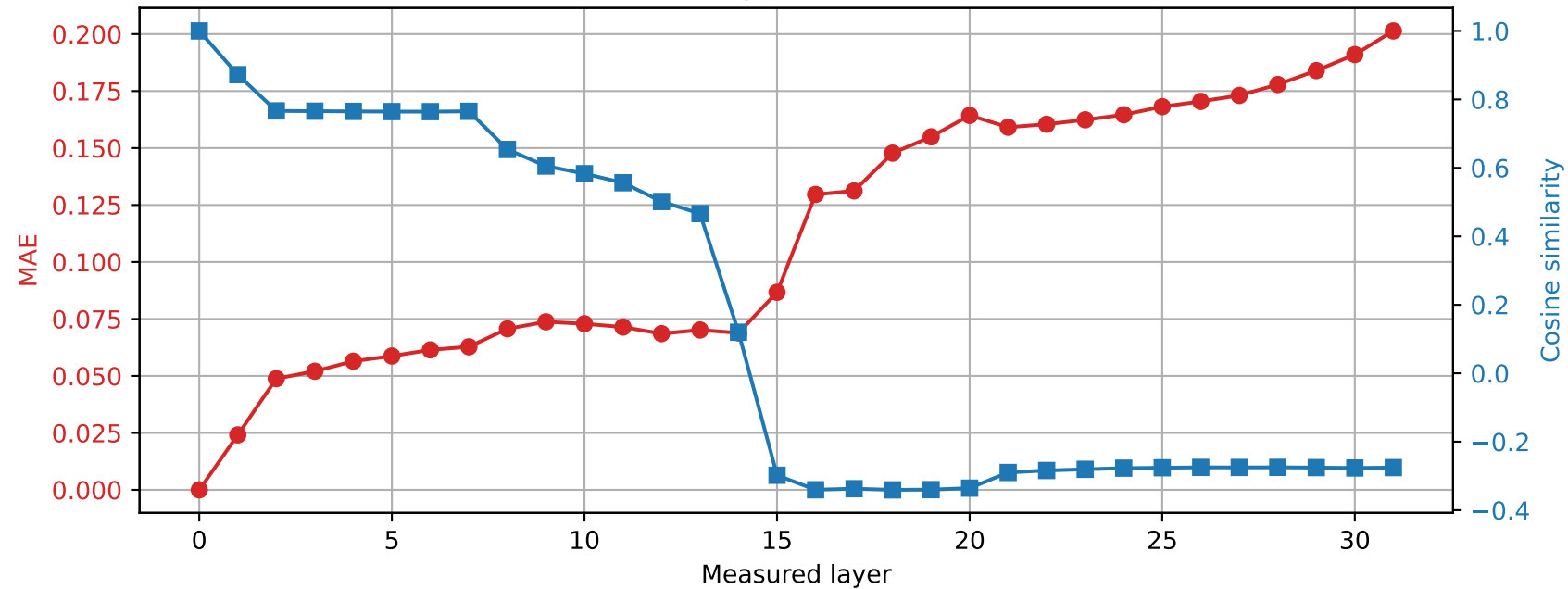
OLMo-7B-hf | Prompt 4 Spared layer 17 | Hybrid vs unquantized
