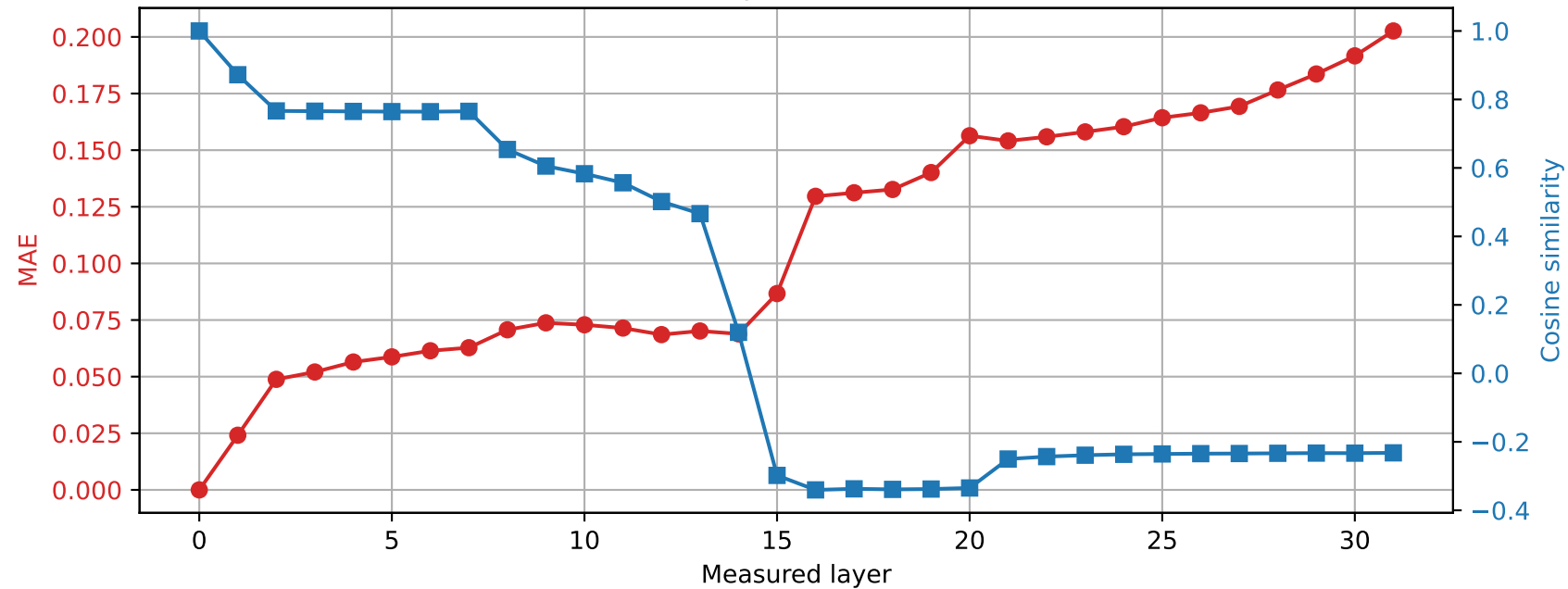
OLMo-7B-hf | Prompt 4 Spared layer 19 | Hybrid vs unquantized
